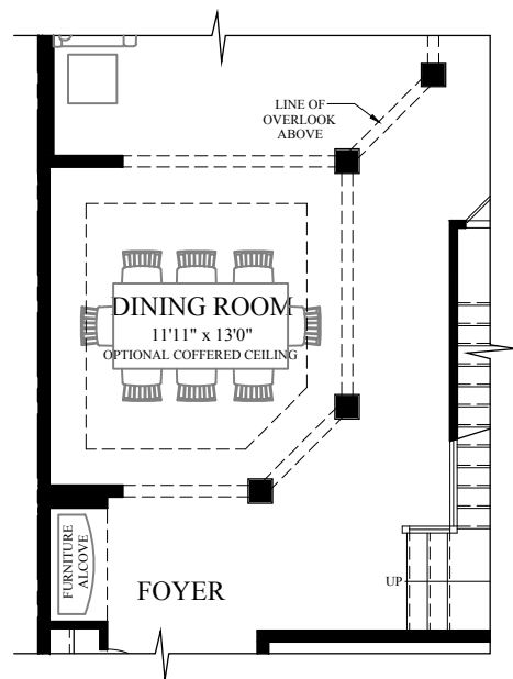
PARTIAL FIRST FLOOR PLAN AT OPTIONAL DINING ROOM
