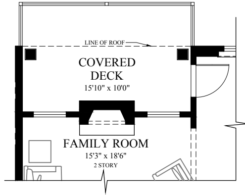
PARTIAL FIRST FLOOR PLAN AT OPTIONAL COVERED DECK
