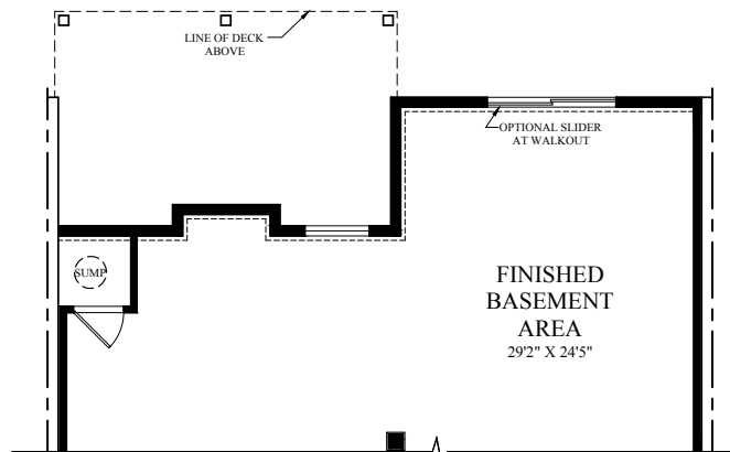
PARTIAL OPTIONAL FINISHED BASEMENT PLAN AT OPTIONAL WALKOUT CONDITION
