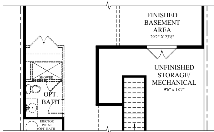
PARTIAL OPTIONAL FINISHED BASEMENT PLAN AT OPTIONAL BATH
